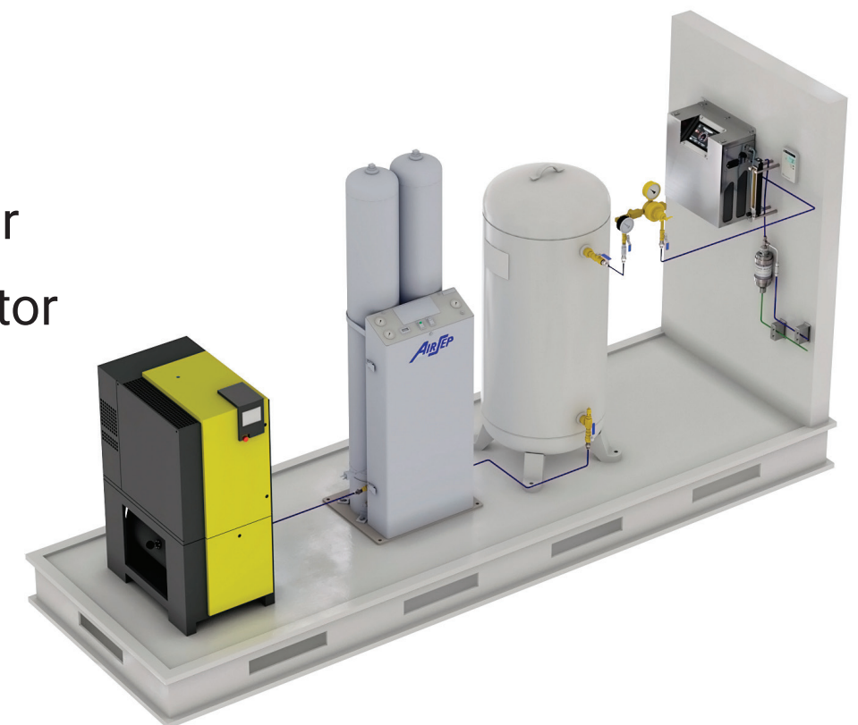
*Typical Installation of the Absolute Ozone® ATLAS 80
