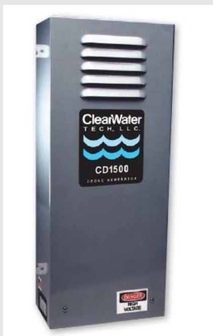
CD1500: 10gm/hr @ 7lpm Oxygen Feed
